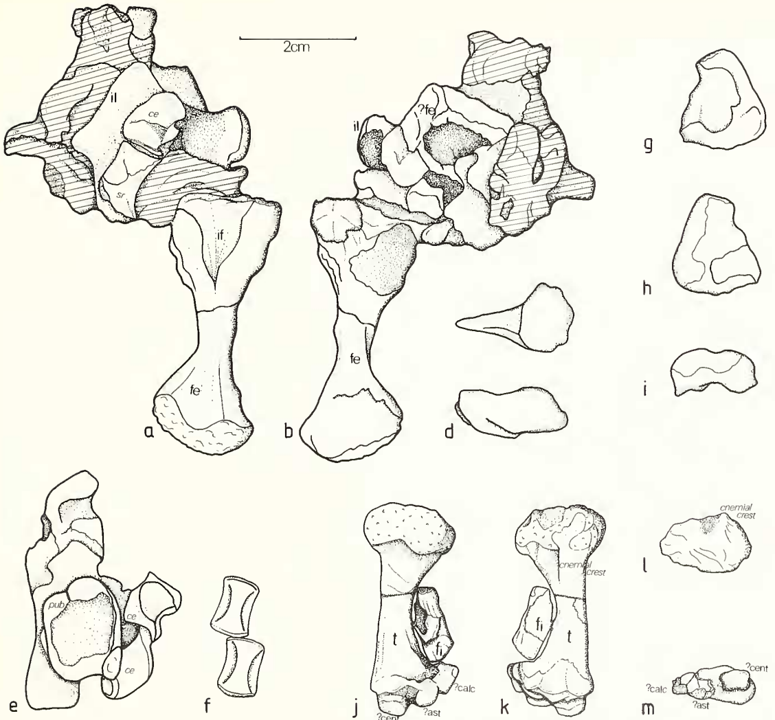
TEXT-FIG. 9. Pelvis and hindlimb elements of juvenile Scaphonyx fisheri (MCZ 1664). a, b , hindlimb and pelvic elements (ilium, sacral vertebra and rib, left femur), in ventral ( a ) and dorsal ( b ) views. c, d , left femur in proximal ( c ) and distal ( d ) views. e, f , pelvic region, showing the right pubis and two caudal vertebral centra in ventral (pubis) and lateral (vertebrae) views ( e ), and in ventral (vertebrae) view ( f ). g-i , distal end of the fragmentary right femur, in ventral ( g ), dorsal ( h ), and distal ( i ) views. j-m , left tibia and fragmentary fibula, in anterior ( j ), posterior ( k ), proximal ( l ), and distal ( m ) views. Some probable tarsal elements are indicated adhering to the distal end of the tibia.
